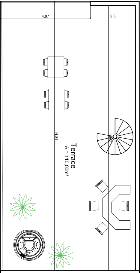
TYPICAL TERRACE PLAN OF END APARTMENT
