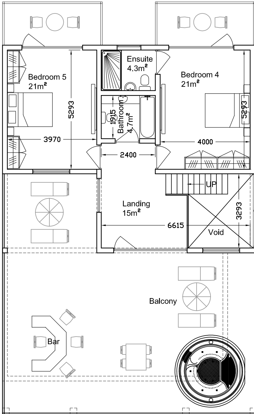
TYPICAL FIRST FLOOR PLAN OF 5 BEDROOM VILLA FLOOR AREA = 66m 2 SCALE 1:100
